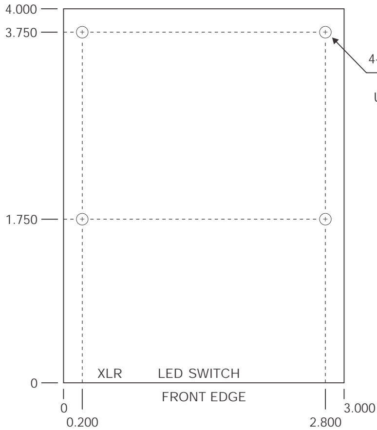
TOP VIEW OF PCB
