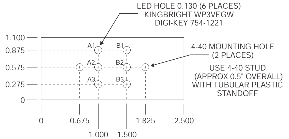
LED DISPLAY PCB
