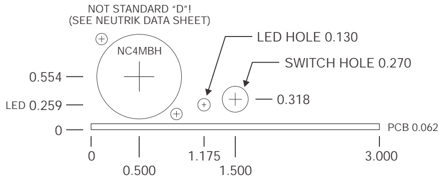
FRONT VIEW FOR PANEL LAYOUT
